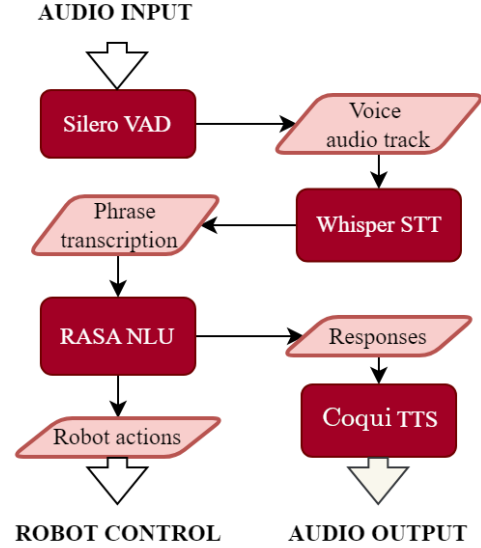
Fig. 4: Voice and language processing systems diagram
