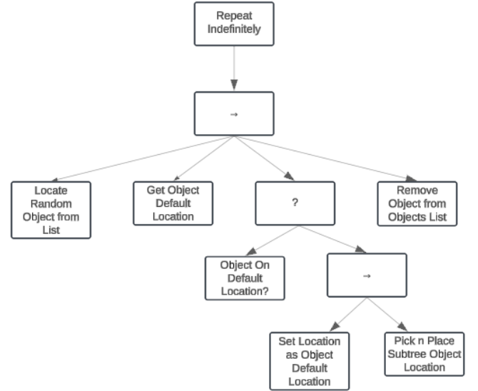
Fig. 1: Simplified Behavior Tree designed to perform pick and place.
