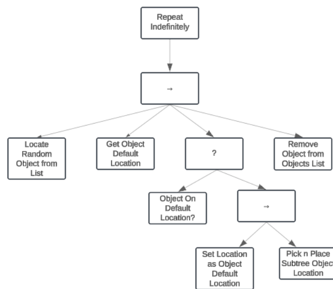
Figure 1. Orchestration of Take Out The Garbage with Behavior Trees
